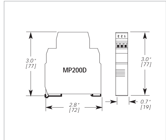
Figure 4 - MP200D dimensions
