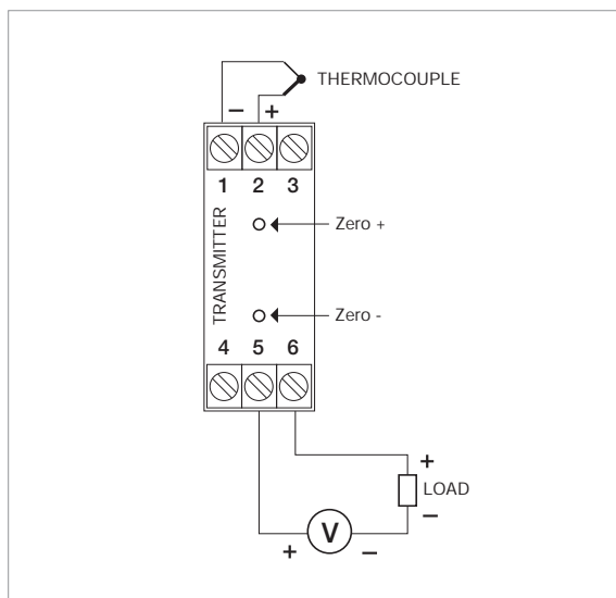
Figure 6 - MP200D wiring (Thermocouple)
