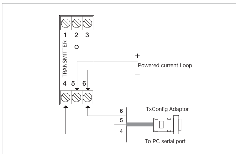
Figure 2 - MP200D-TxConfig Adaptor wiring (loop powered). Terminal 5 is left opened.
