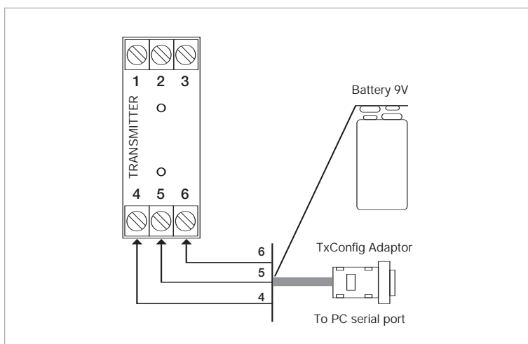
Figure 1- Adaptor connections to the MP200D
